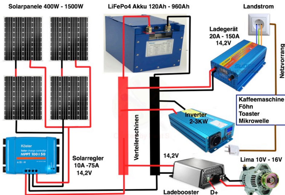
Connection Overview (24V plants, double voltage)
