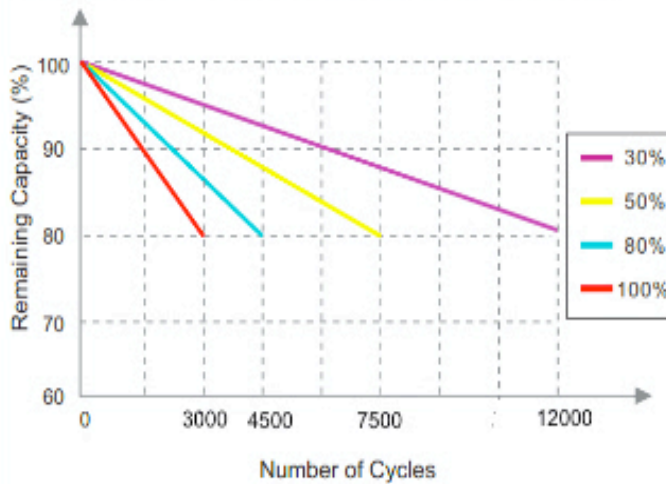
Different DOD Discharge Cycle Life Curve @1C
